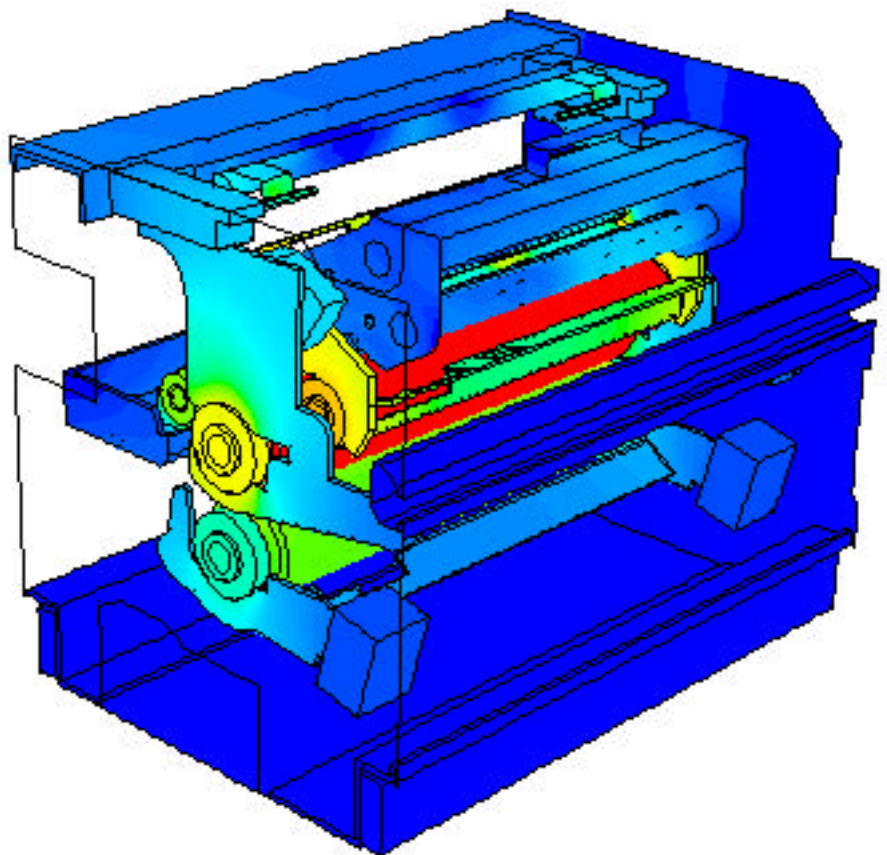
Figure 1: Temperature distribution of the fuser system viewed from paper exit. (Some components removed for clarity.)
