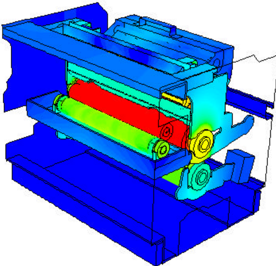
Figure 2: Temperature distribution of the fuser system viewed from the paper entrance. (Some components removed for clarity.)
