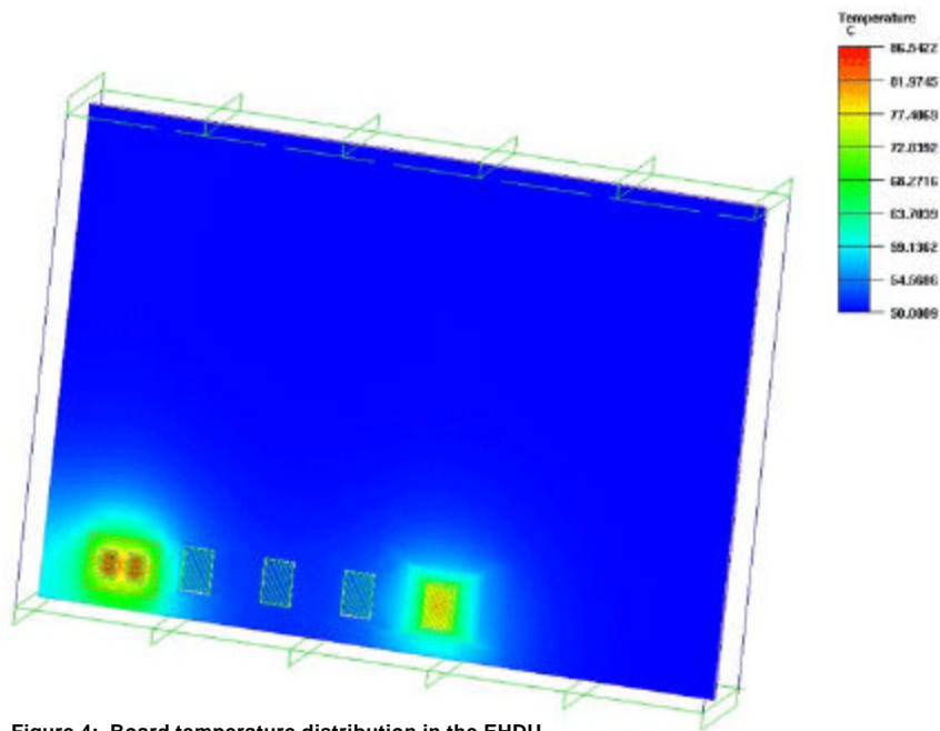
Figure 4: Board temperature distribution in the EHDU
