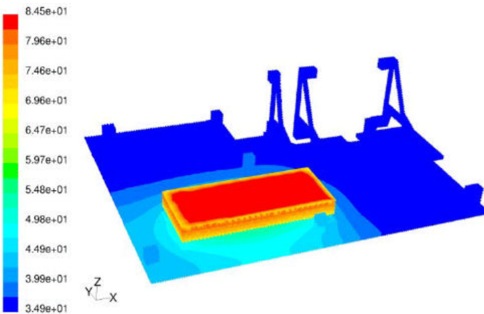
Figure 2: Temperature distribution inside the motor control module
